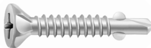
Ponta broca com asa Punta broca con alas Self-drilling point with wings
